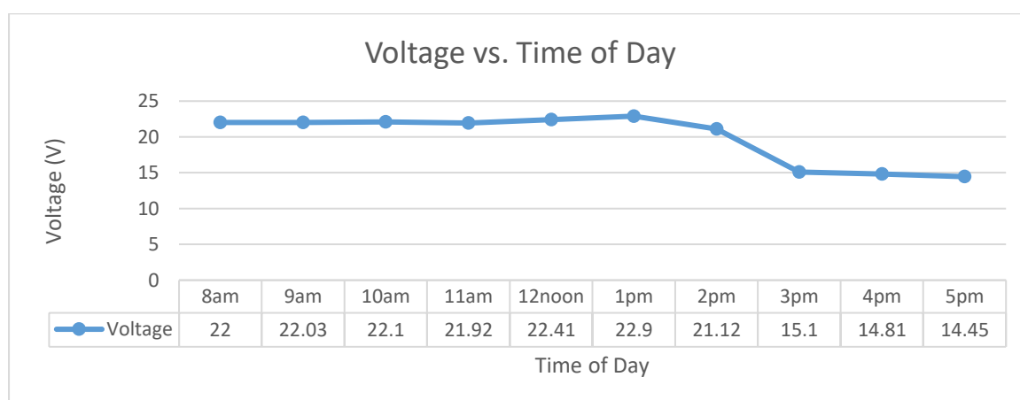
Figure 4.1 Open-circuit Voltage Test versus Day Time
