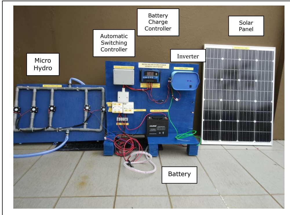
Figure 3.2 The Prototype of Micro Solar-Hydro Power Generation System
