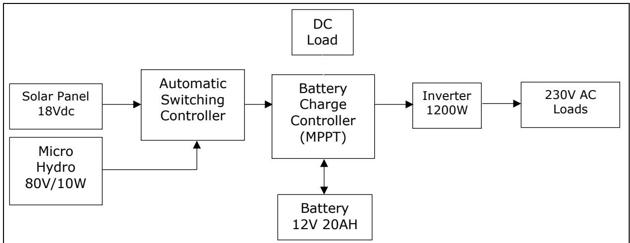
Figure 3.1 Block Diagram of Micro Solar-Hydro Power Generation System
